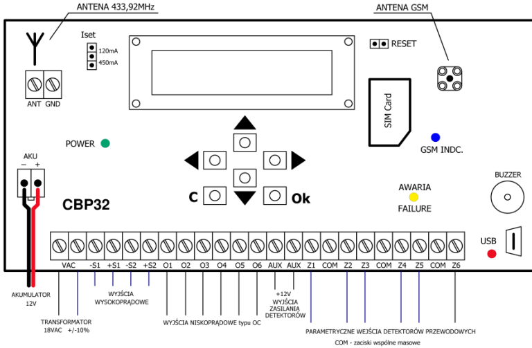
Diagram 2. Connection of wired detectors with CBP32 control panel supporting intruder alarming as well as detection of anti-sabotage box opening, wires cut or short circuit.
